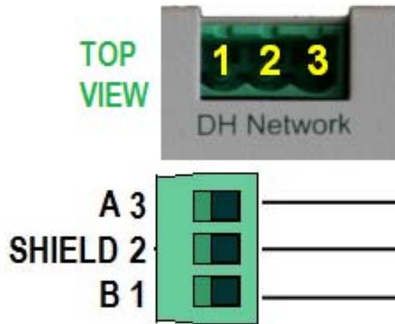
Equustek products DH485 connector, pin 1 is on the side of power connector
