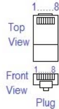
Allen Bradley RJ45 DH485 connector
