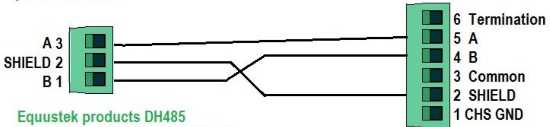
Equustek products DH485 connector, pin 1 is on the side of power connector
